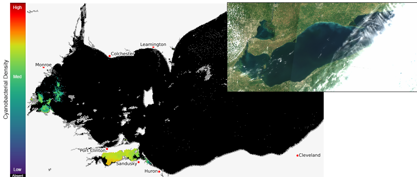
Current Lake Erie Sentinel-3 satellite imagery from the Ocean and Land Color Imager (OLCI) on Jul 07, 2023, showing bloom location and extent in the western basin. Grey indicates clouds or missing data. The estimated threshold of cyanobacteria detection is 20,000 cells/mL. Inset shows a truecolor image of the entire lake. Data derived from Copernicus Sentinel-3.
