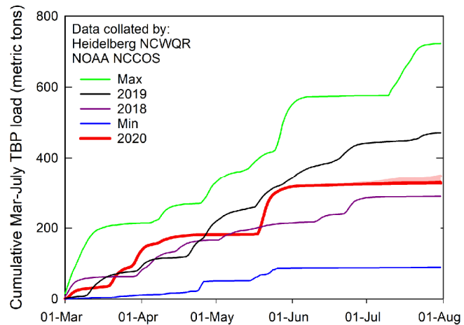
Figure 2. Cumulative total bioavailable phosphorus (TBP) loads for the Maume River (based on Waterville). Each line denotes a different year. 2020 is in red, the solid line is the measured load to June 22 the red area shows the likely range for the remainder of the loading season, and the light red shows the possible range.
