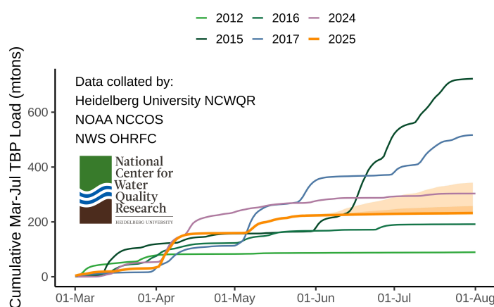
Fig. 2. Cumulative TBP loads for the Maumee River (Waterville, OH). Each line denotes cumulative load for different years. 2025 is in orange: the solid line is the measured load to May 27 and predicted load for the rest of the loading season (thru July); the orange shading shows the possible load range for the remainder of the season.
