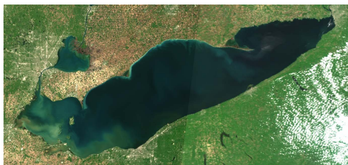
Fig. 4. True color image for 16 May 2025 derived from the Copernicus Sentinel-3a/b satellite. Sediment from recent high river flow produces brown and tan water in the western basin.
