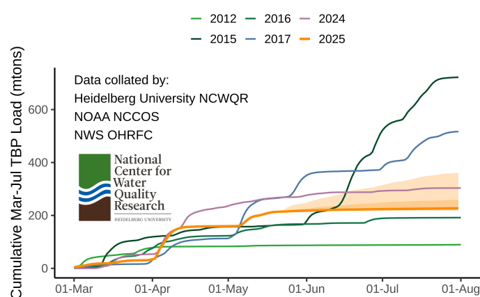
Fig. 2. Cumulative TBP loads for the Maumee River (Waterville, OH). Each line denotes cumulative load for different years. 2025 is in orange: the solid line is the measured load to May 21 and predicted load for the rest of the loading season (thru July); the orange shading shows the possible load range for the remainder of the season.
